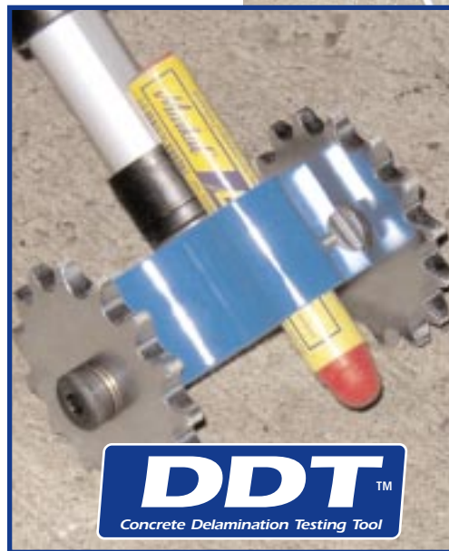
Delamination Detection Tool shown with attached crayon for on-the-spot marking of delaminated areas.
